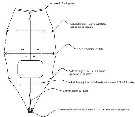
Typical cross section through Fuselage
