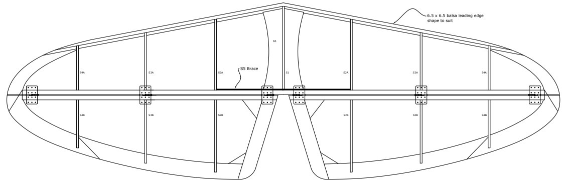
Tailplane and Elevator Build flat on table
